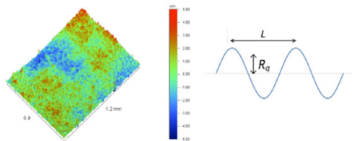
Figure 2: Typical 3D representation of a surface profile (left) and graphic clarification of parameters R_q and L (right), which are used to describe surface roughness.
