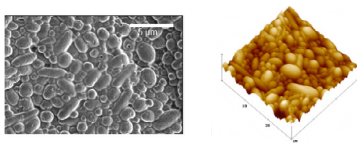
Figure 1: SEM image and a 3D AFM image of a Covestro softfeel coating, illustrating the particles in the size range of approximately 1–10 micrometers.
